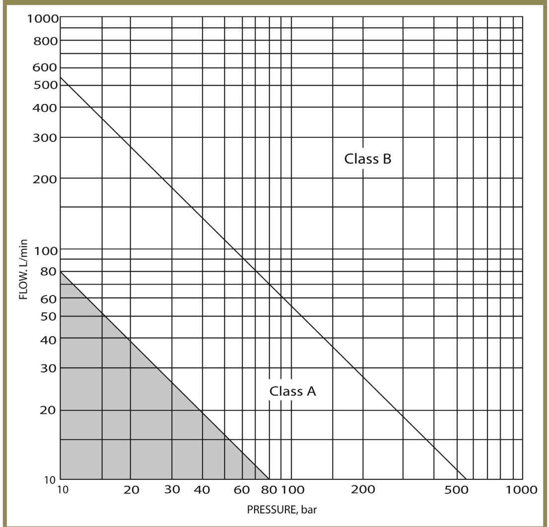
FIGURE 10 Pressure flow chart
